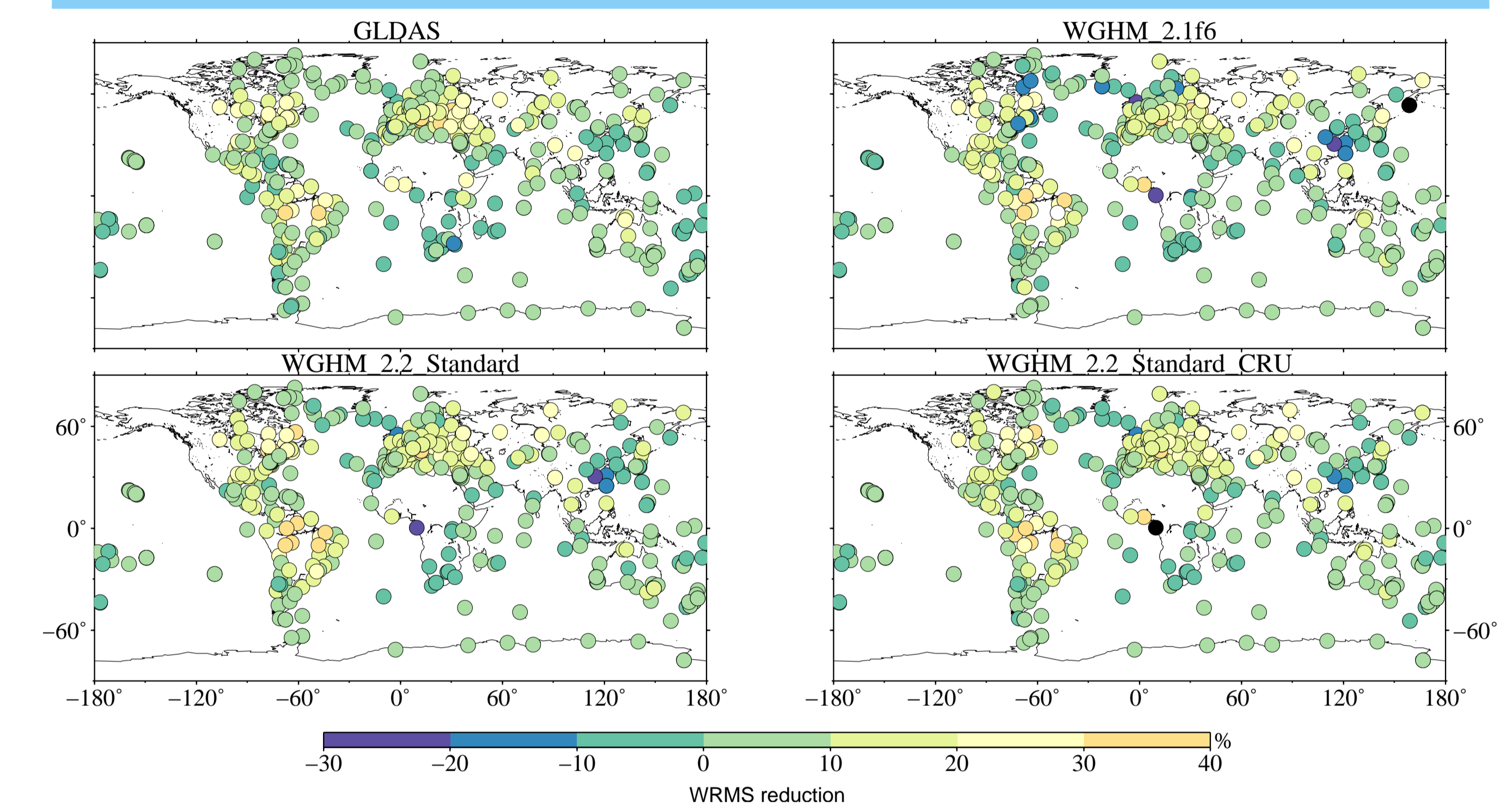
Figure 3: WRMS reductions between the ITRF2014 solutions and the four hydrological models at selected common stations. The same color scheme as Figure 1 (right) is applied here but limited up to the maximum 40%. WRMS reductions between two other GNSS solutions with the four hydrological models are not shown here.
